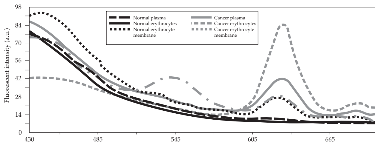
Figure 1. Emission spectra of plasma, erythrocytes, erythrocyte membrane from normal and cancer samples on excitation at 400 nm.
