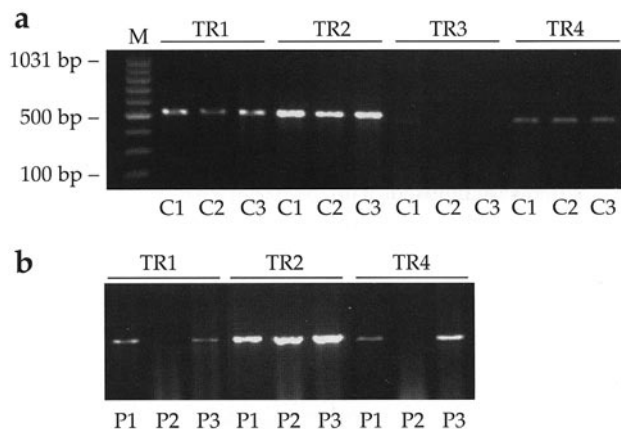
Figure 1. Expression pattern of TRAIL receptors in blood mononuclear cells from normal subjects (a) and leukemia patients (b). P1 and P2 are patients with a positive t(9;22) translocation, while P3 is translocation-negative. Note that no TRAIL-R1 and -R4 expression is detected in P2. M, molecular size marker; bp, base pairs; C, control; P, patient
