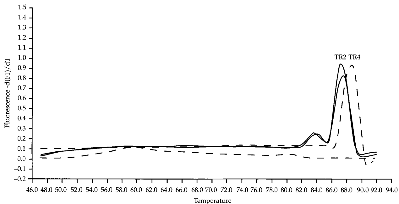
Figure 2. Analysis of the expression of TRAIL receptors by real-time PCR. After completing the amplification, melting curves were generated by increasing the temperature gradually from 45 °C to 95 °C with continuous measurement of fluorescence. The curves were then converted to melting peaks by plotting the negative derivate of the fluorescence with respect to temperature ( -dF/dT ) against temperature. Shown are TRAIL-R2 and -R4 from two patients with CML. Note that TRAIL-R4 was not expressed in one of the patients.
