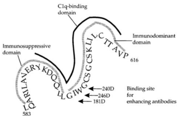
Figure 1. Schematic representation of interaction of the HIVenv 583-616 domain of the transmembrane glycoprotein 41 with C1q and some anti-HIV antibodies.
