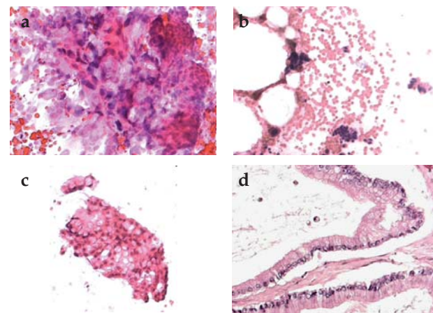
Figure 2. Brush cytology of mucinous carcinomas. (a) Moderately differentiated mucinous carcinoma. HE, 200x. (b) Smear from poorly differentiated infiltrative mucinous carcinoma with small discohesive clusters with macronuclei (asterisk). HE, 200x. (c) Intraductal papillary mucinous neoplasm. HE, 200x. (d) Biopsy of differentiated, infiltrative papillary mucinous carcinoma. HE, 200x.
